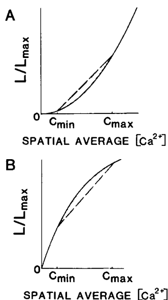
FIGURE 2. Limits on the error in the estimate of spatial average [Ca^{2+}] . Solid curves are hypothetical calibration curves ( I_n ). Dashed lines (Eq. 5) provide limits on the extent to which spatial average [Ca^{2+}] can be underestimated ( A ) or overestimated ( B ). Shaded regions represent all possible relationships between L/L_{max} and spatial average [Ca^{2+}] when [Ca^{2+}] in the preparation is bounded by C_{min} and C_{max} . A : case when d^2I_n(C)/dC^2 > 0 . B : case when d^2I_n(C)/dC^2 < 0 .
